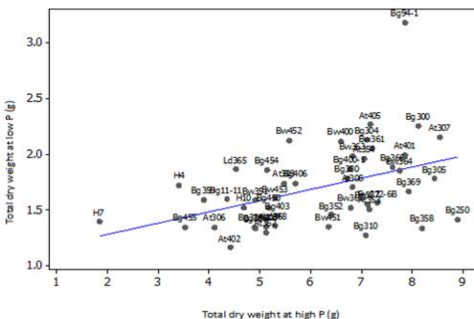
Figure 5. Varietal performances on dry weight gained at low P vs high P availability at 52 days after planting.
