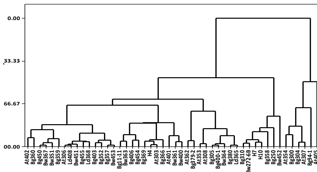
Figure 2. Dendrogram constructed by using shoot and root dry weights, number of tillers and shoot P concentration and contents at 10 \mu M P supply
