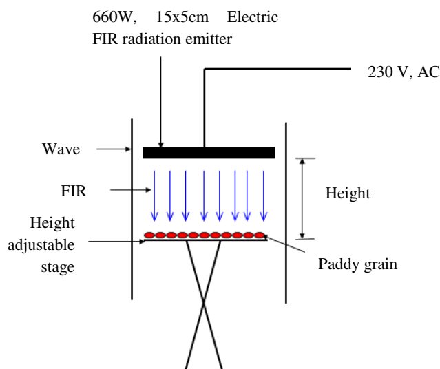
Fig. 1. Schematic diagram of the experimental apparatus for gelatinization of rough rice using FIR radiation
