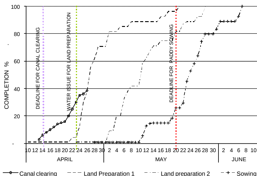
Fig. 8. Progress of land preparation
