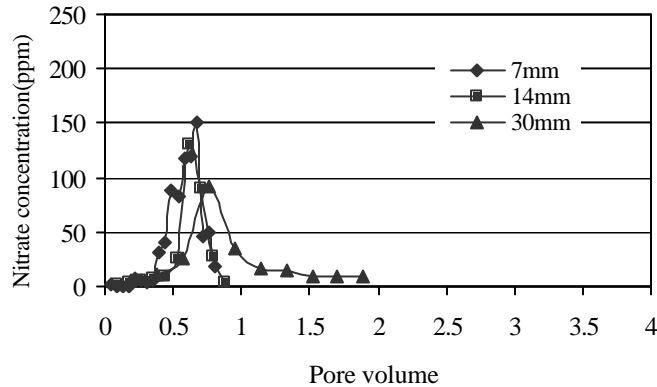
Fig.5. Nitrate breakthrough curves in 40 cm column at 70 kg N/ha.
