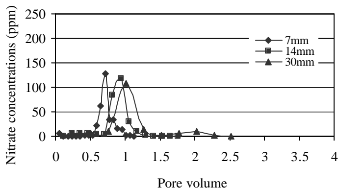
Fig. 3. Nitrate breakthrough curves in 30 cm column at 70 kg N/ha.
