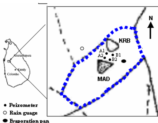
Fig. 1. Schematic diagram of the TCS and the location of measuring equipments.
