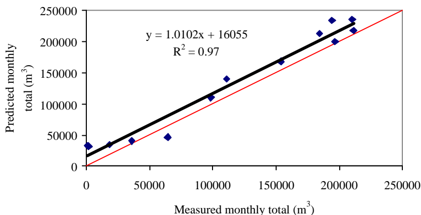
Fig. 6. Monthly simulated and observed volume of water in the KRB tank.
