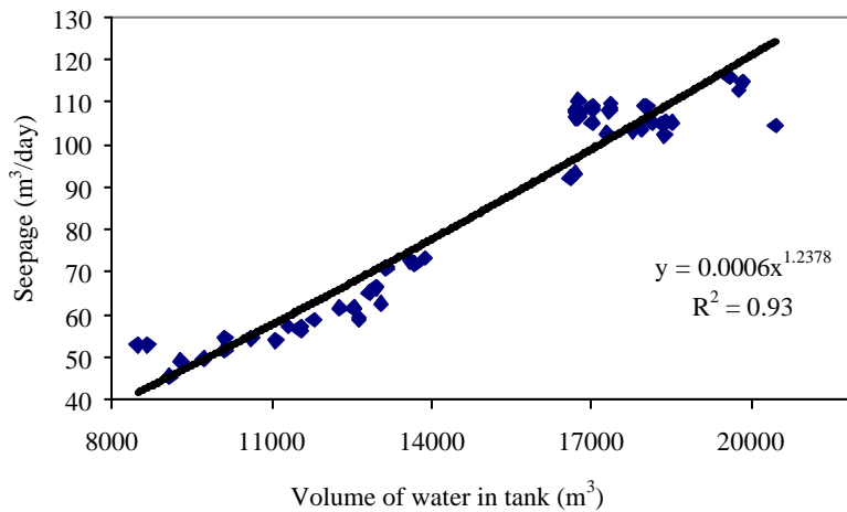
Fig. 2. Relationship between tank volume and seepage in the MAD tank.
