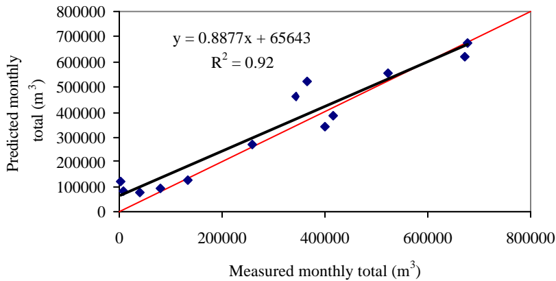
Fig. 5. Monthly simulated and observed volume of water in the MAD tank.
